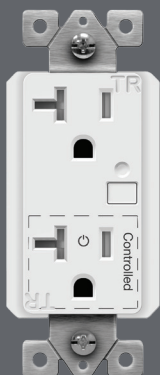
HALF-CONTROLLED 20A TAMPER-RESISTANT DECORATOR RECEPTACLE PL20R
